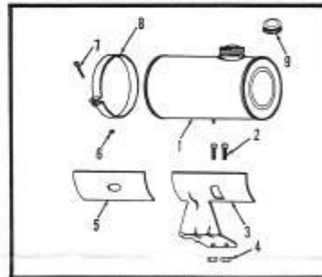
FUEL TANK
