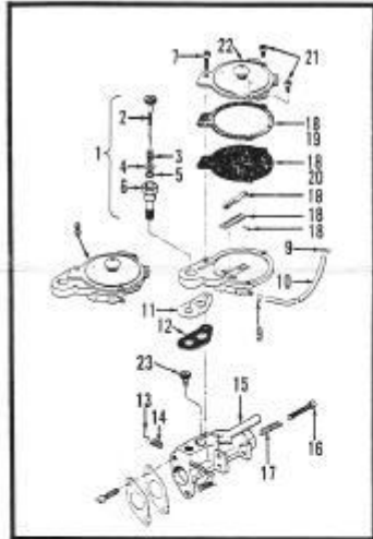
CARBURETOR
